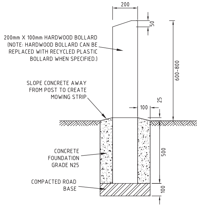
BUSHLAND BOLLARD TYPE 1
