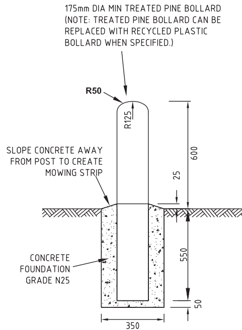
PEDESTRIAN BOLLARD TYPE 1
