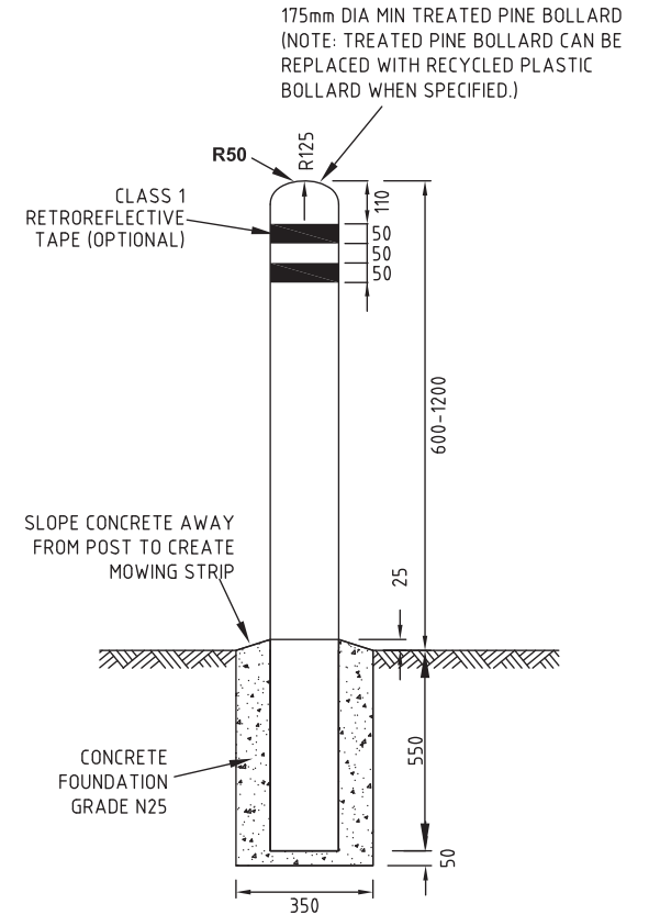
PEDESTRIAN BOLLARD TYPE 2
